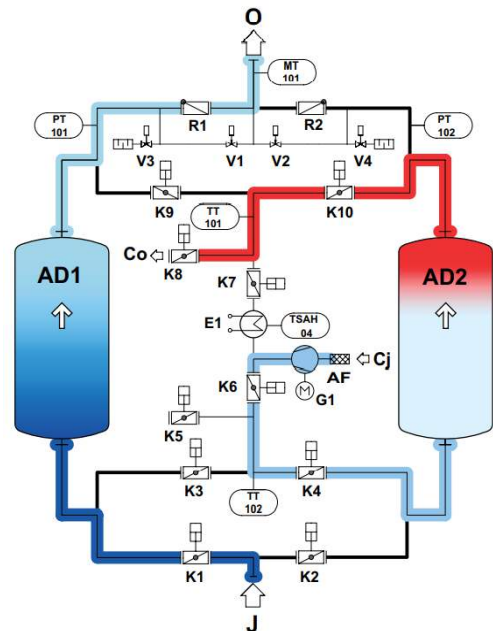
Drying + Cooling Phases
