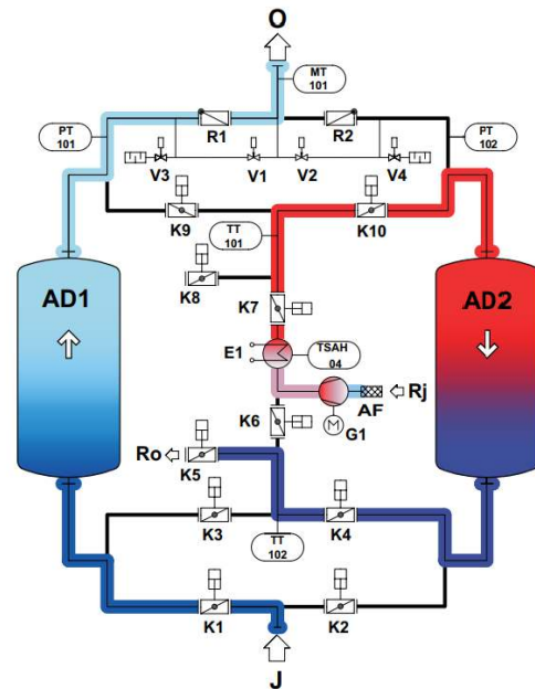
Drying + Heating Phases
